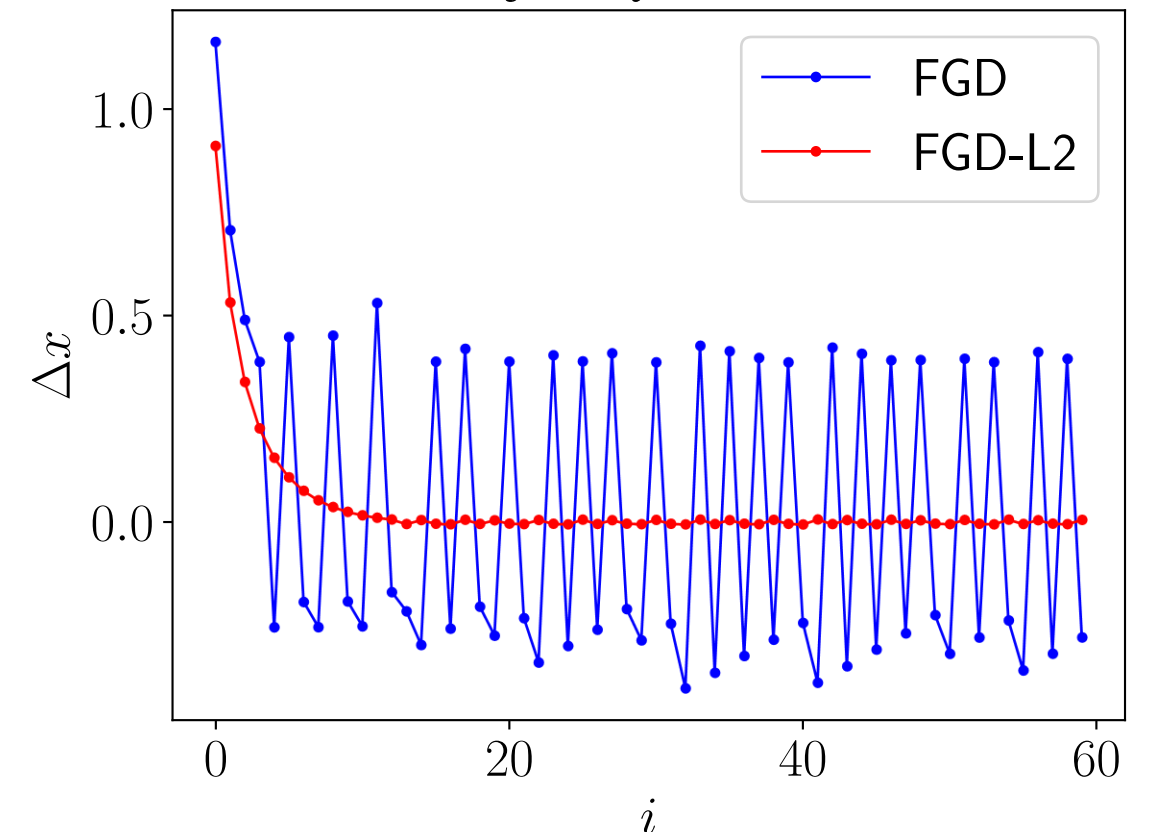
(f) Trajectory of \Delta x at \alpha = 0.1
