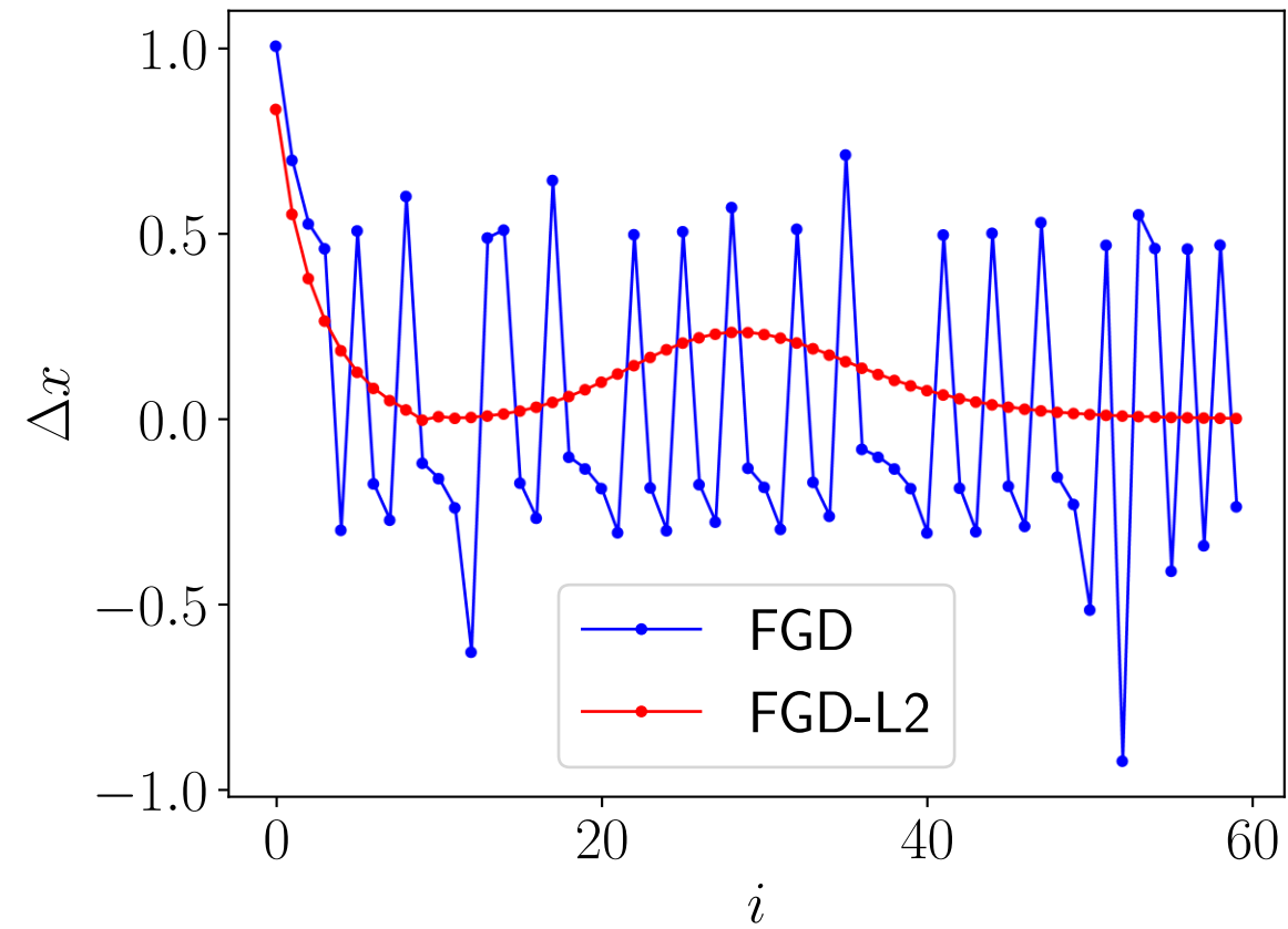
(e) Trajectory of \Delta x at \alpha = 0.3
