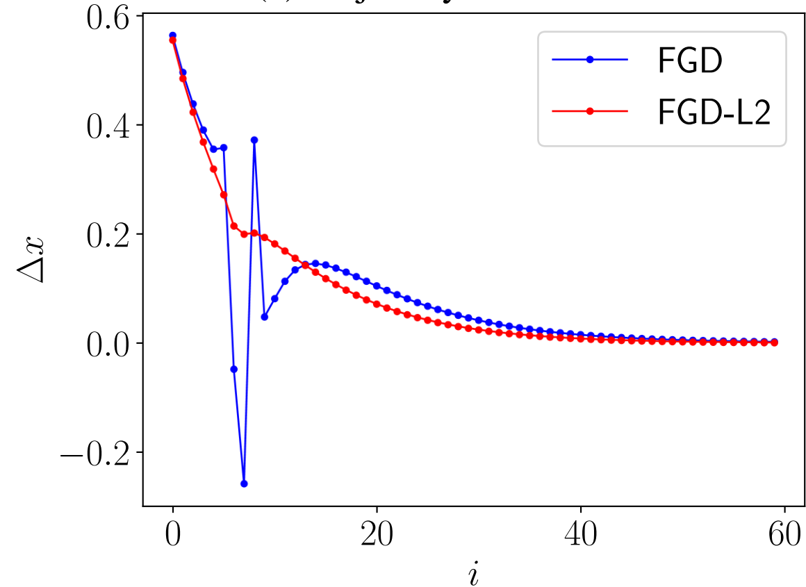
(b) Trajectory of \Delta x at \alpha = 0.9
