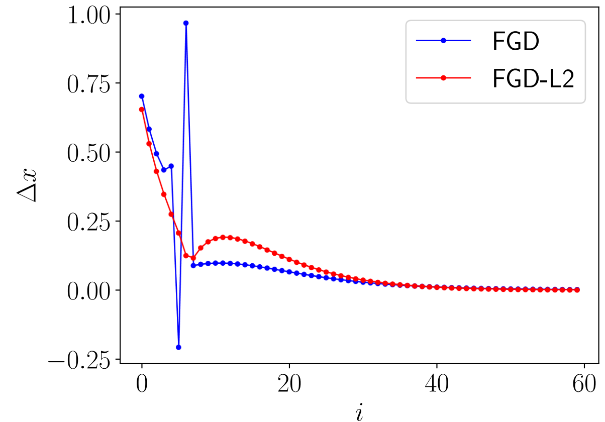
(c) Trajectory of \Delta x at \alpha = 0.7
