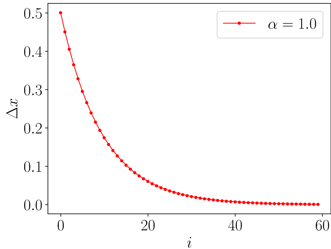
(a) Trajectory of \Delta x at \alpha = 1.0
