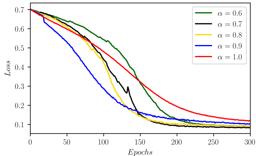
(a) Training set convergence trajectories of DIJ
