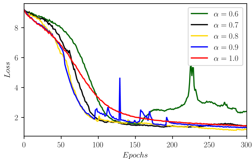
(d) Training set convergence trajectories of ETTh1
