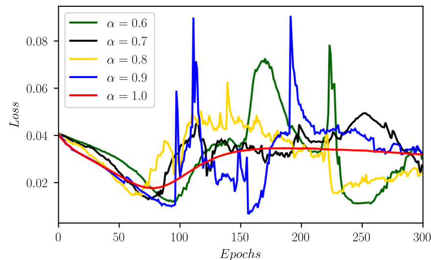
(e) Validation set convergence trajectories of ETTh1
