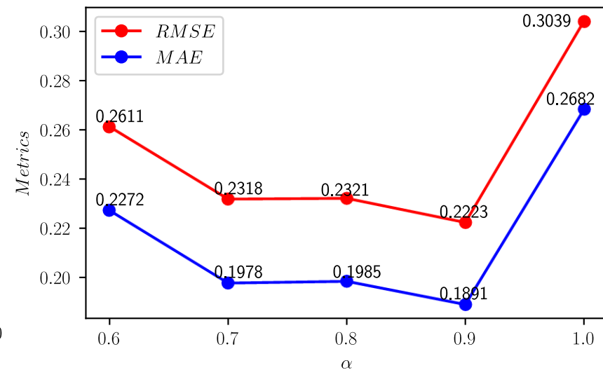
(c) Test set quantization results of DIJ
