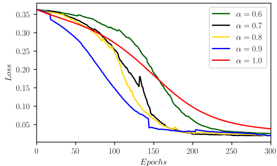
(b) Validation set convergence trajectories of DIJ
