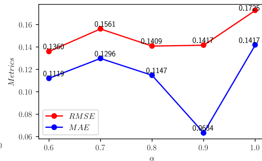
(f) Test set quantization results of ETTh1
