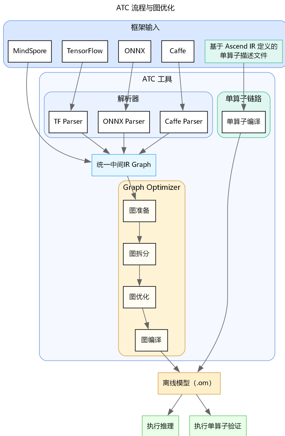
Figure 2.1: ATC 框架图
