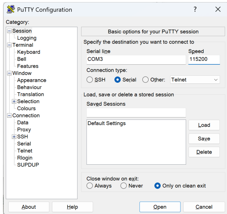
Figure 46.: PUTTY
