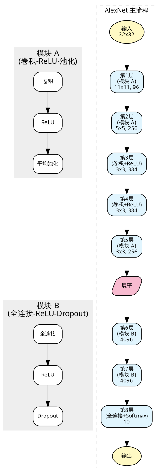
Figure 3.7.: AlexNet
