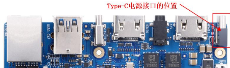
Figure 40.: TYPE-C Power
