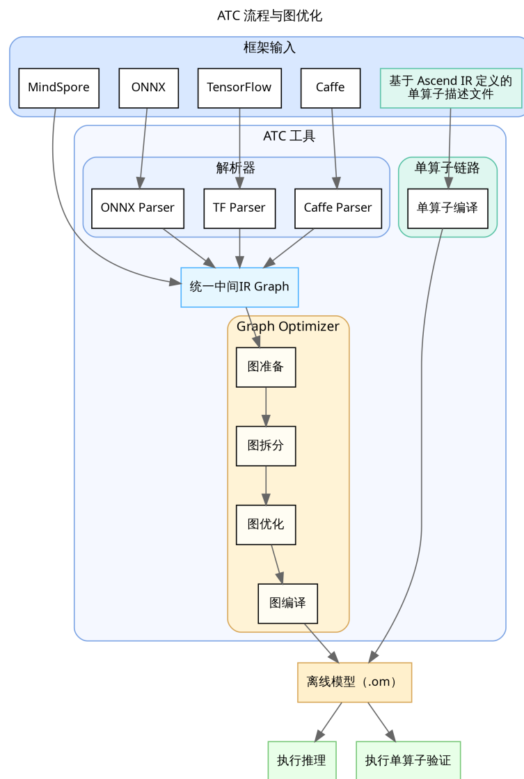
Figure 2.3.: ATC 框架图
