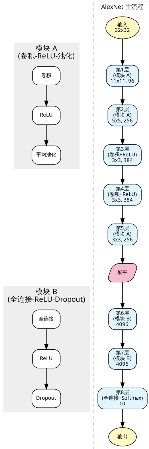
Figure 3.7.: AlexNet
