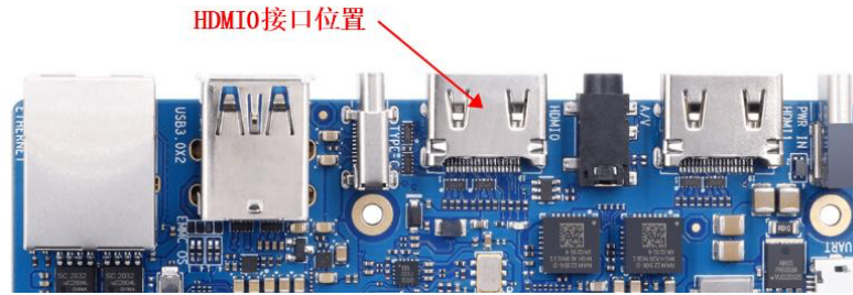
Figure 39.: HDMI0
