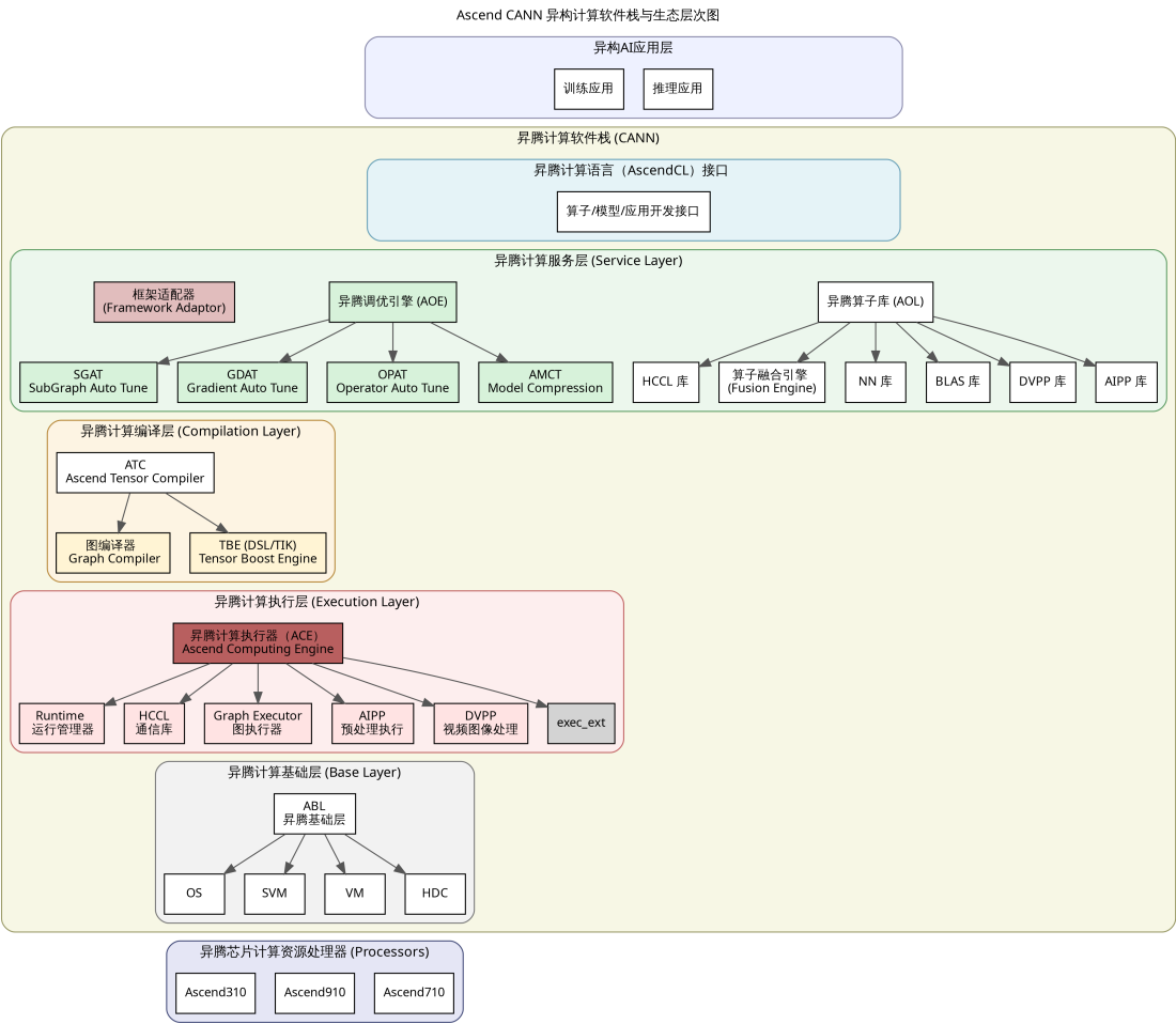
Figure 2.1.: CANN 架构图
