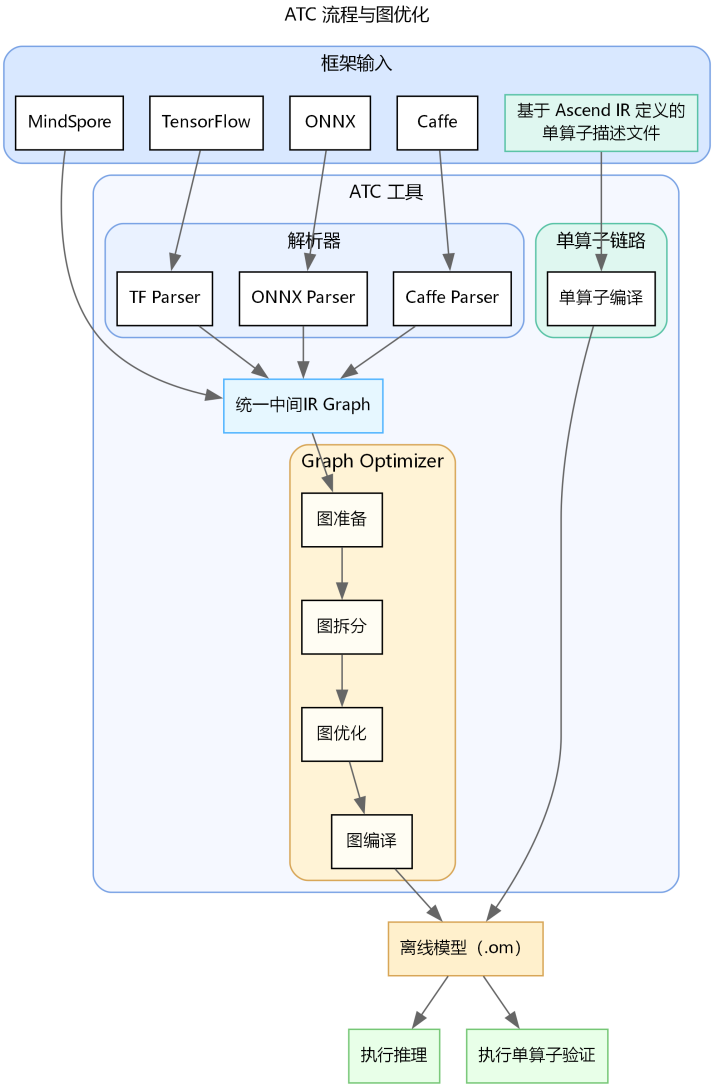
Figure 2.3: ATC 框架图
