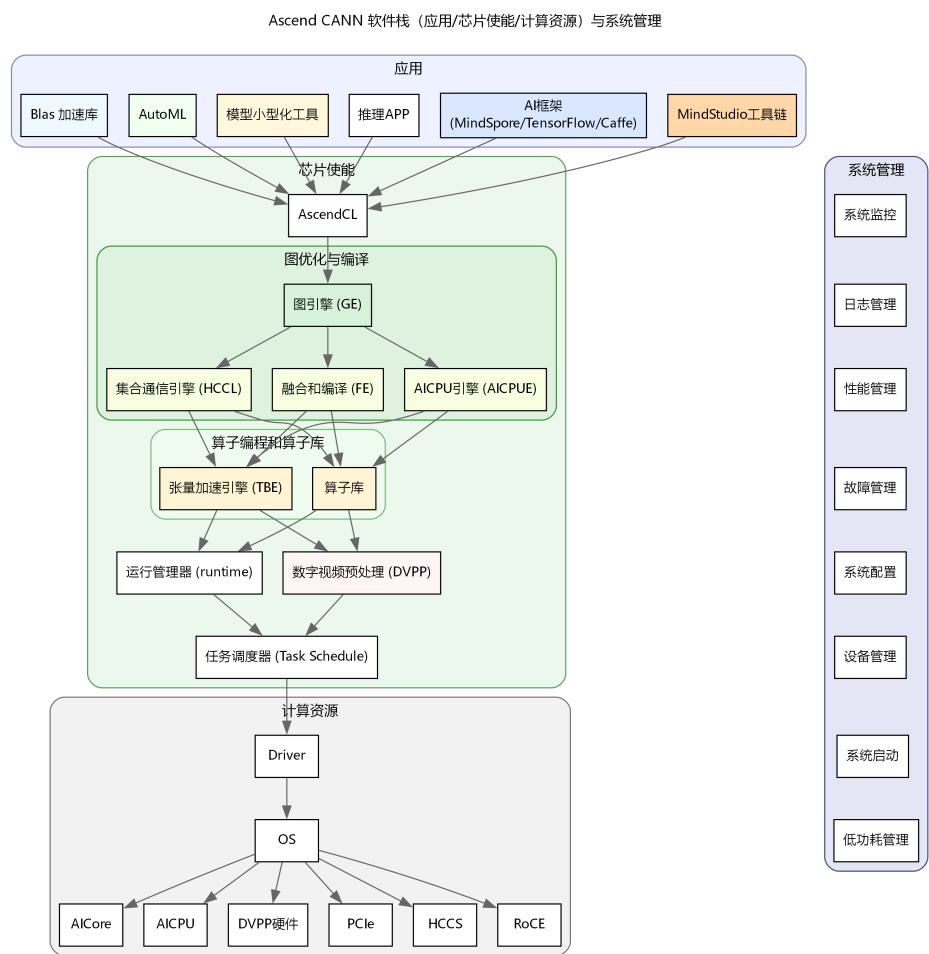
Figure 2.2: CANN 架构图
