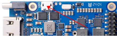
Figure 44.: MicroUSB 串口
