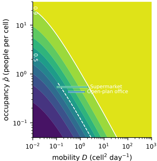
(a) \beta q = 0.5 \text{ day}^{-1}
