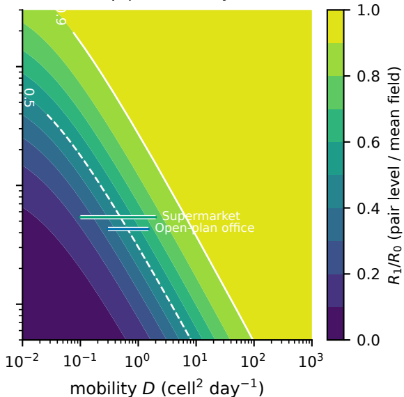
(b) \beta q = 1.25 \text{ day}^{-1}
