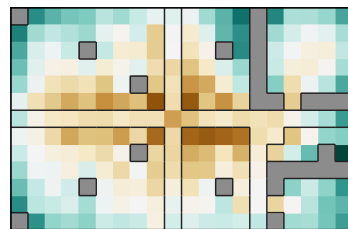
(c) 模拟
