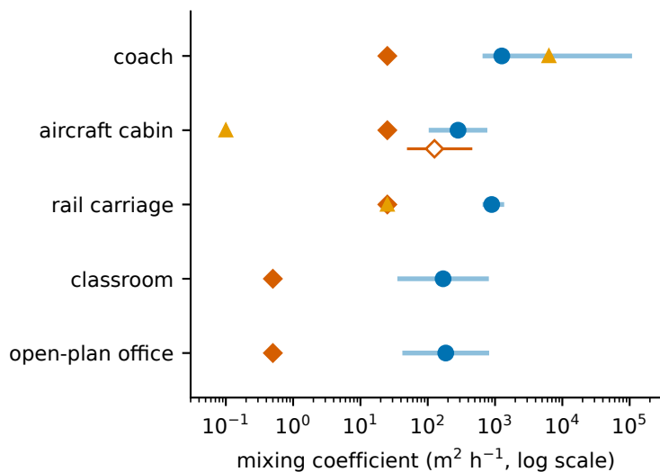
(d) Measured and fitted coefficients
