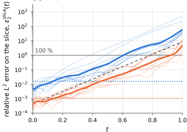
(a) random
