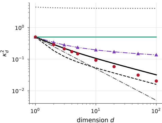
(a) bounds of the constant
