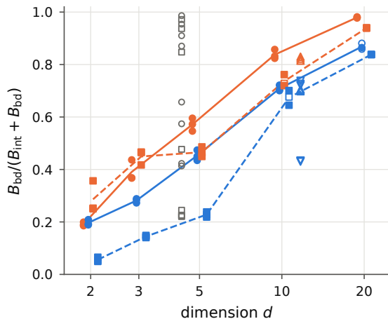
(c) boundary share of the bound
