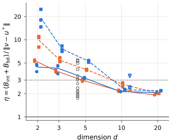
(b) efficiency of the bound
