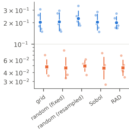
Wave 2D
