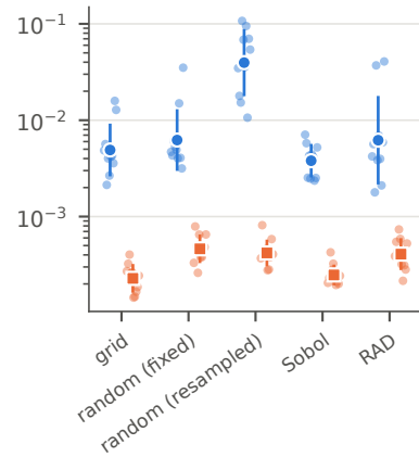
Laplace 2D
