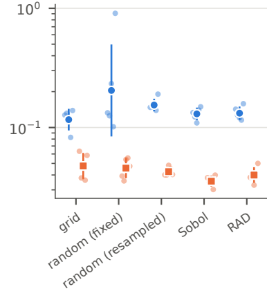
Laplace 3D
