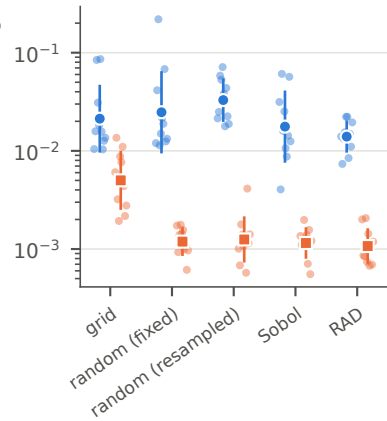
Heat 1D
