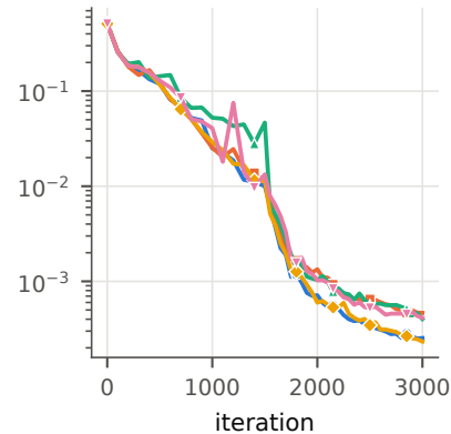
Laplace 2D
