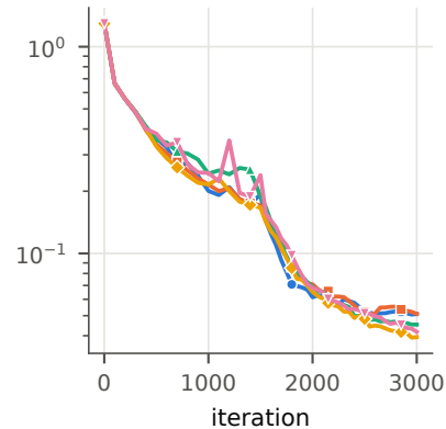
Laplace 3D
