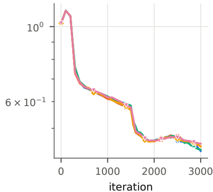
Wave 1D ( c = 2 , two modes)
