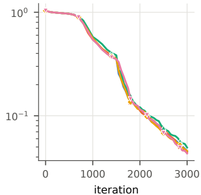
Wave 2D
