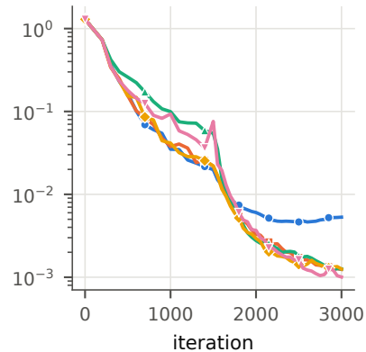
Heat 1D
