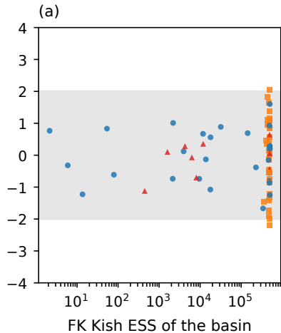
basin mass z (FK – DK)
