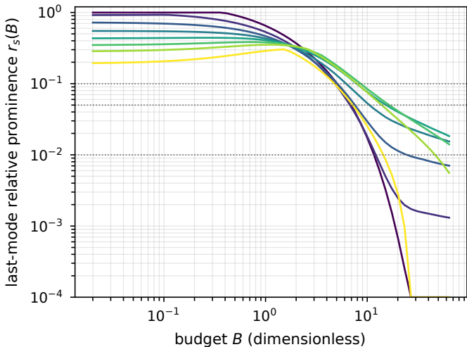
m = 2 , smoothed exact law (bandwidth 0.04)
