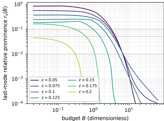
m = 3 , smoothed exact law (bandwidth 0.04)
