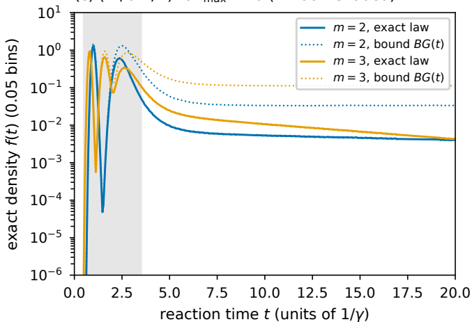
(c) (m, 0.1, 1) to t_{\max} = 20 (window shaded)
