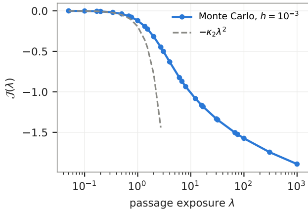
(c) corrected mass law
