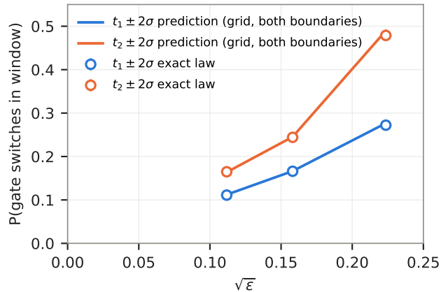
(b) the \sqrt{\varepsilon} switching law
