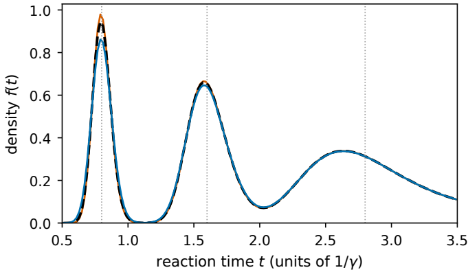
m = 3, \varepsilon = 0.1, B = 1 (mode counts: 3, 3, 3)
