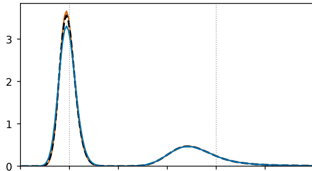
m = 3, \varepsilon = 0.1, B = 4 (mode counts: 2, 2, 2)
