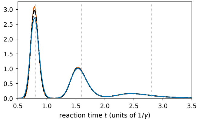
m = 3, \varepsilon = 0.1, B = 4 (mode counts: 2, 2, 2)
