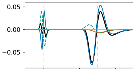
(c) m = 3, \varepsilon = 0.1, B = 1
