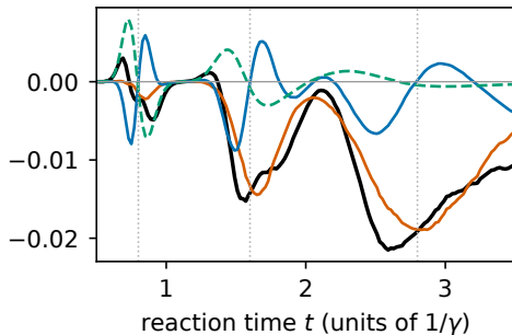
(c) m = 3, \varepsilon = 0.1, B = 1
