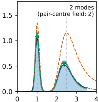
(c) m = 2, \varepsilon = 0.1
