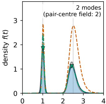
(a) m = 2, \varepsilon = 0.05
