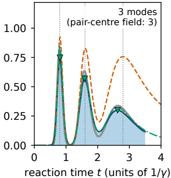
(b) m = 3, \varepsilon = 0.1
