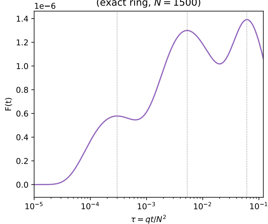
(d) two shortcuts, three peaks (exact ring, N = 1500 )
