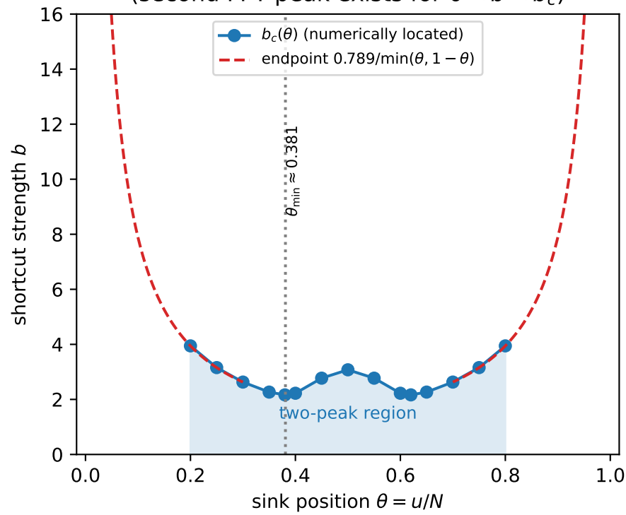
(a) saddle-node phase boundary b_c(\theta) (second FPT peak exists for 0 < b < b_c )
