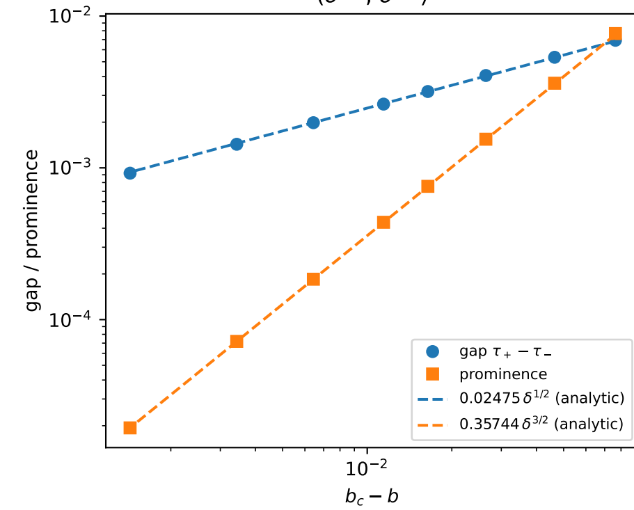
(c) normal-form fold scaling ( \delta^{1/2} , \delta^{3/2} )
