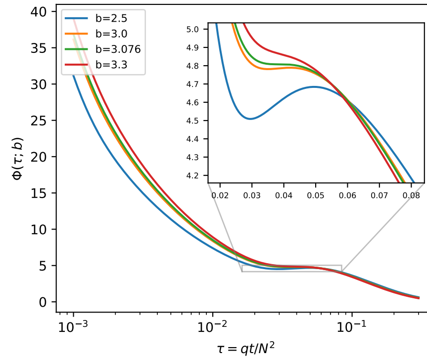
(b) master curve \theta = \xi = 1/2 : second peak annihilates at b_c = 3.0764
