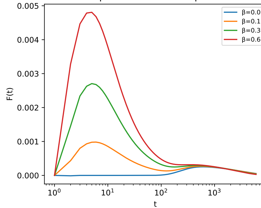
(e) 2D torus ( 31 \times 31 ): capture + late interior peaks
