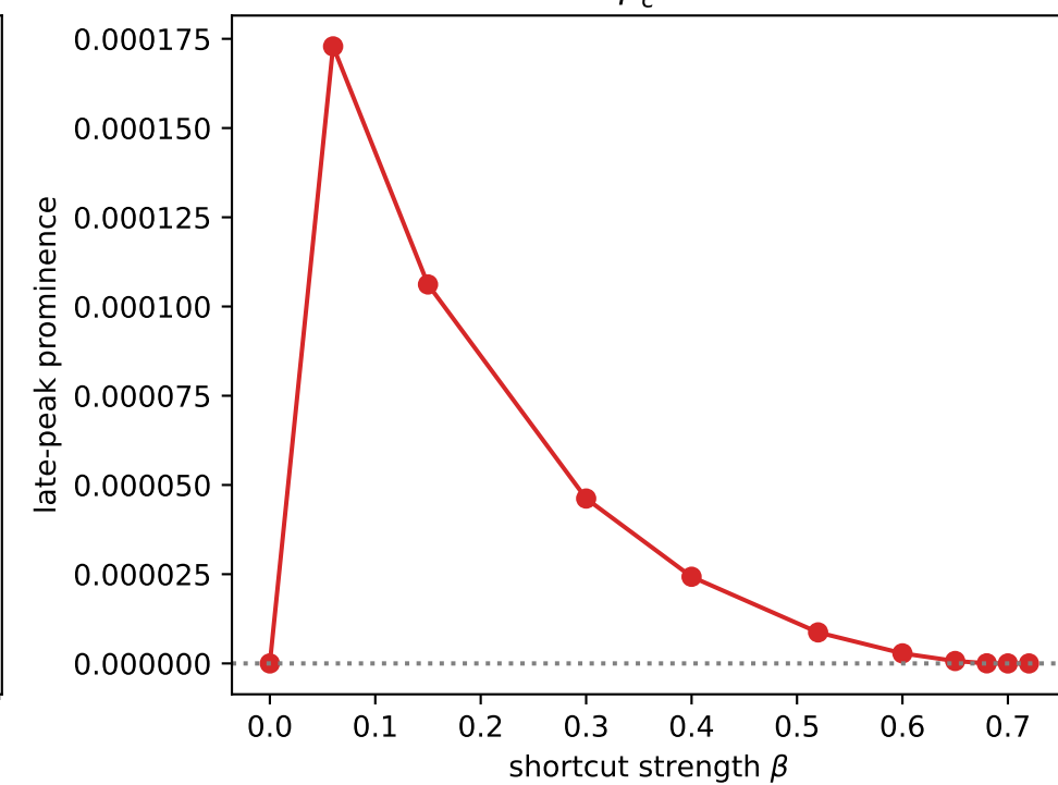
(f) 2D fold: late-peak prominence \rightarrow 0 at \beta_c^{2D} \approx 0.69
