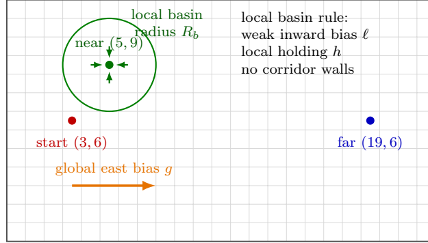
Figure 5: Configuration for the local-bias basin test. The geometry remains a plain reflecting rectangle. The added mechanism is a local near-target basin, not a corridor.
