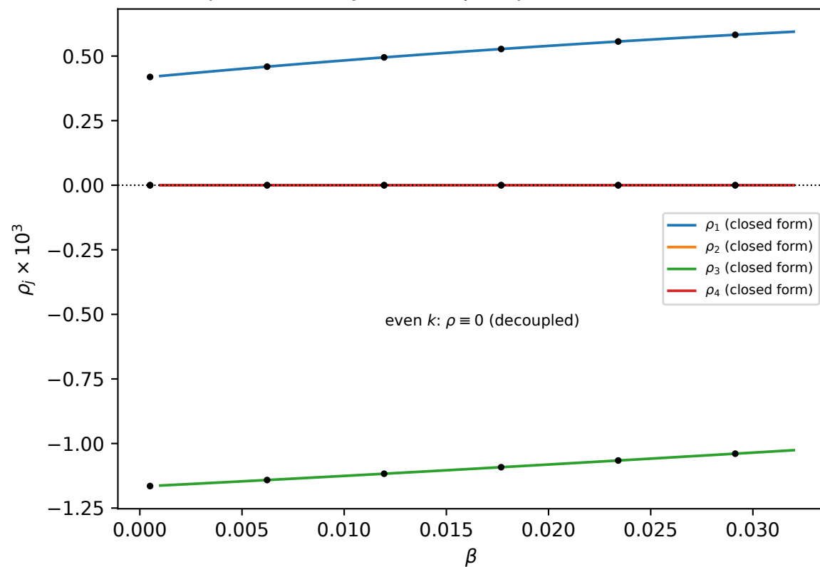
(3) the amplitudes carry ALL the \beta -dependence ( N=100 , start u+4 )
