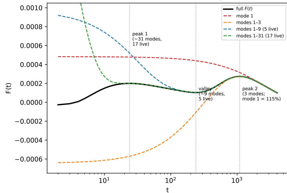
(4) which terms build the curve ( N=100 , \beta=0.01 , d=4 )
