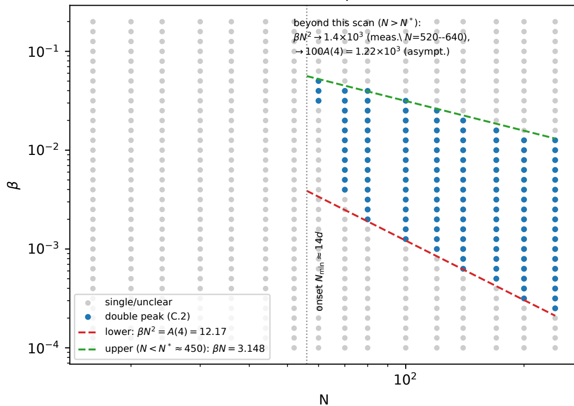
(1) where the double peak lives ( d=4 )
