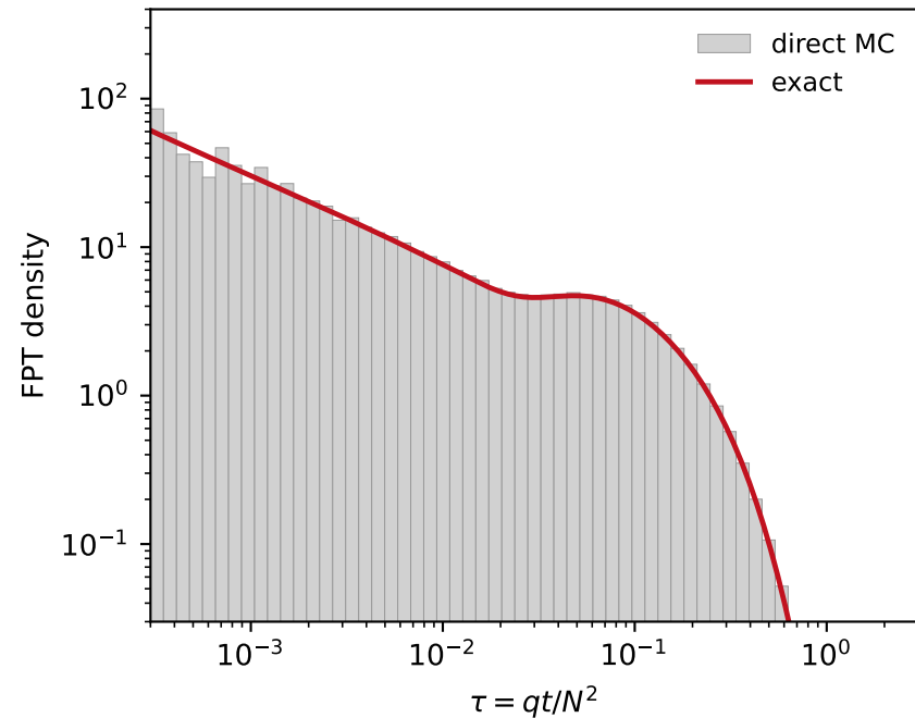
(a) direct simulation vs exact ( \theta = 1/2 , b = 2.6 < b_c )
