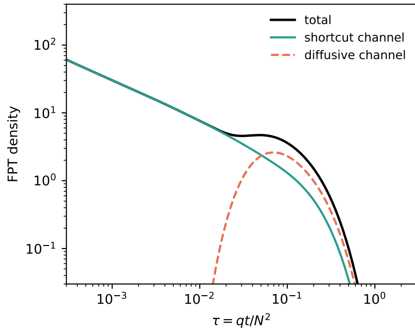
(b) channel resolution (early=shortcut, late=diffusive)
