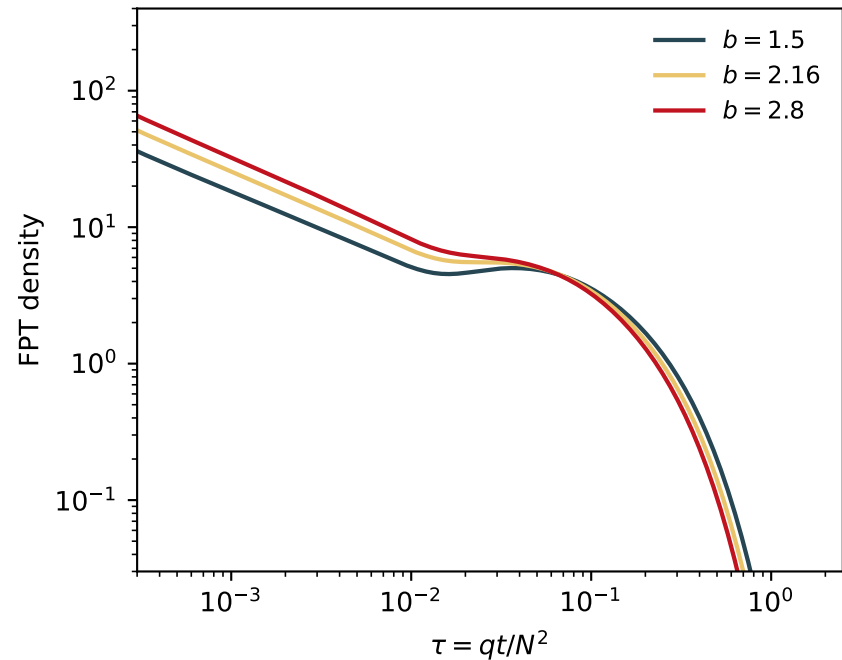
(c) non-antipodal \theta = 0.38 across b_c(\theta) \approx 2.16
