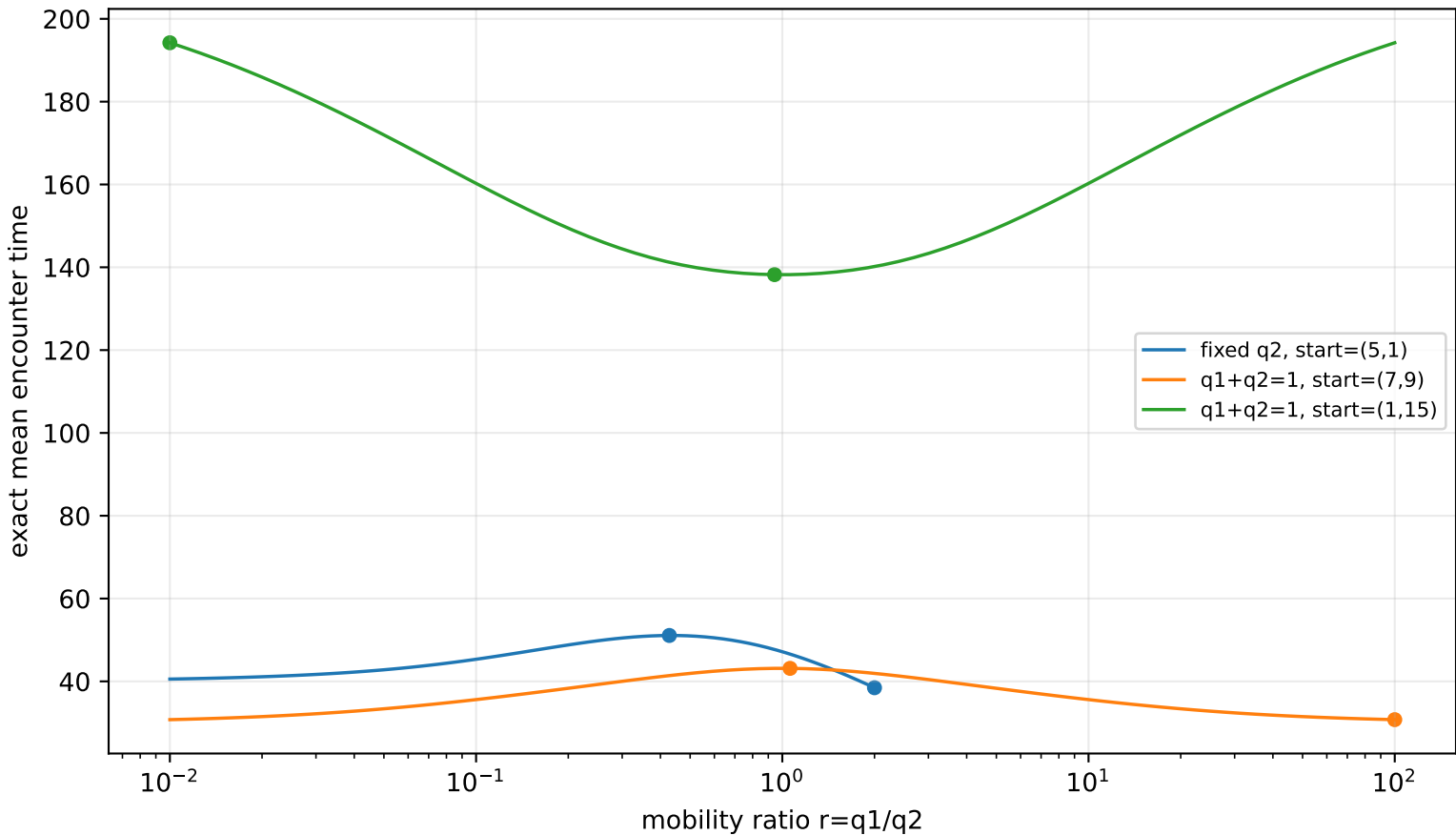
mean first-encounter time versus mobility ratio
