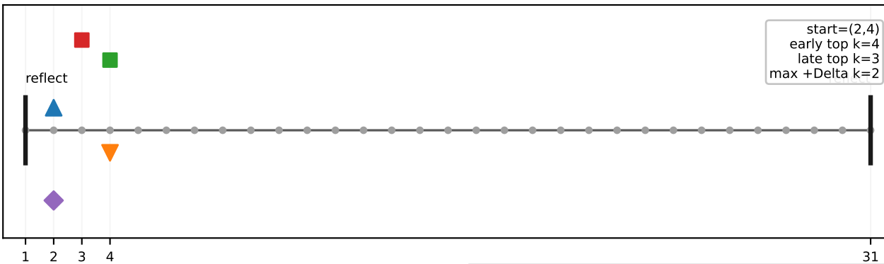
E_target_shift_2_4: physical lattice 1..31
