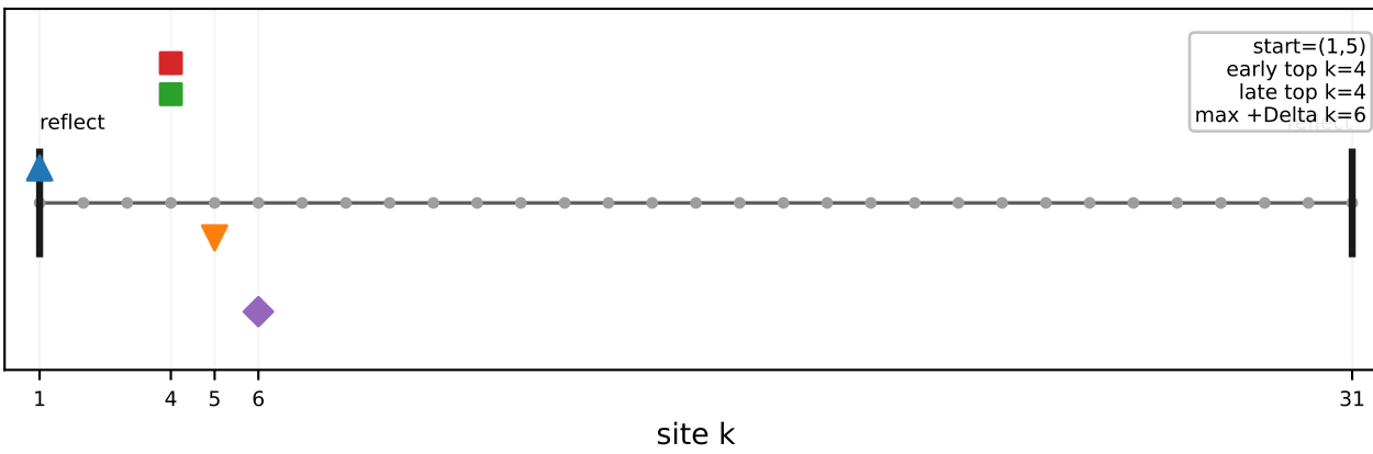
B_boundary_1_7: physical lattice 1..31
