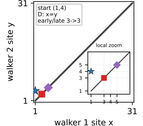
state space O plus absorbing diagonal D
