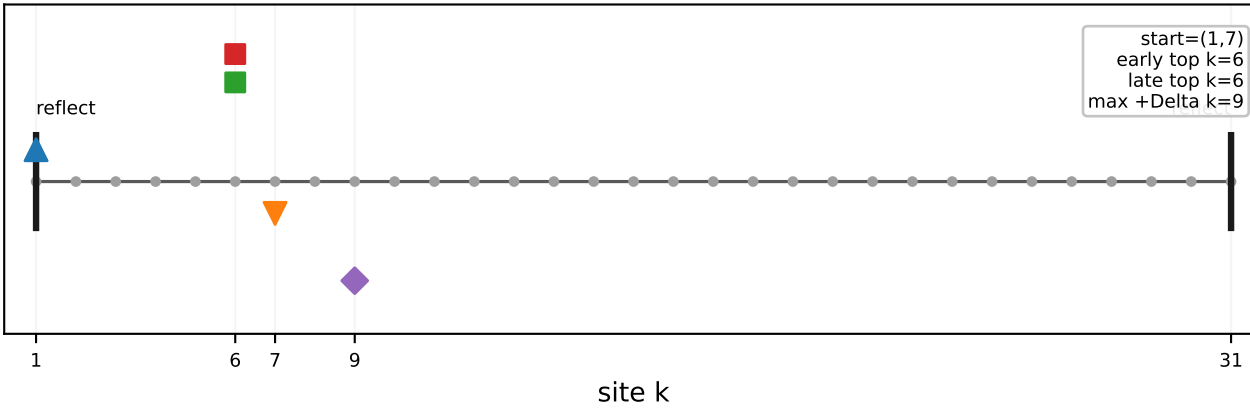
C_boundary_1_4: physical lattice 1..31
