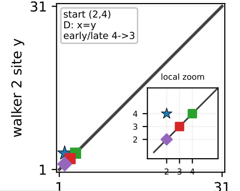
state space O plus absorbing diagonal D
