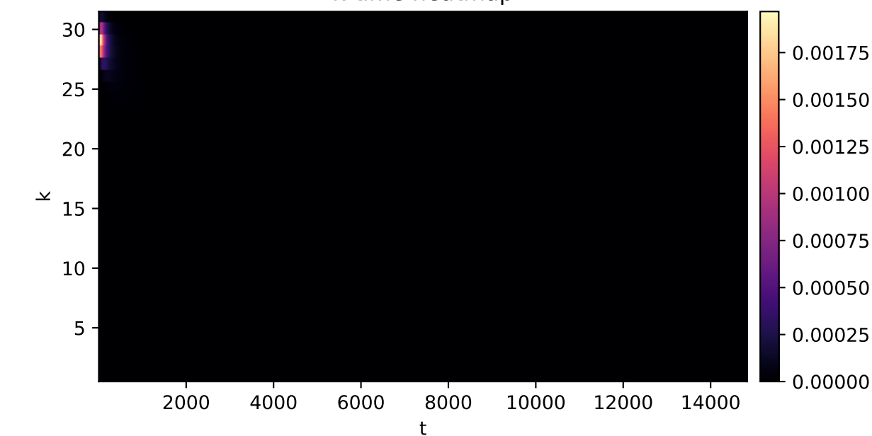
crossing comparison
