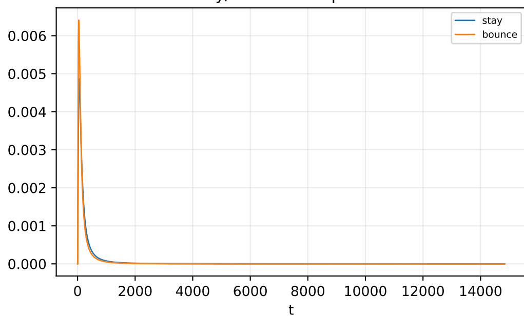
stay/bounce comparison
