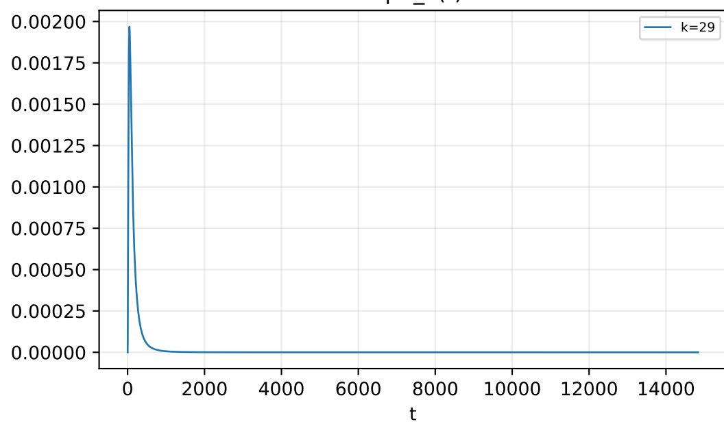
early/late C_k
