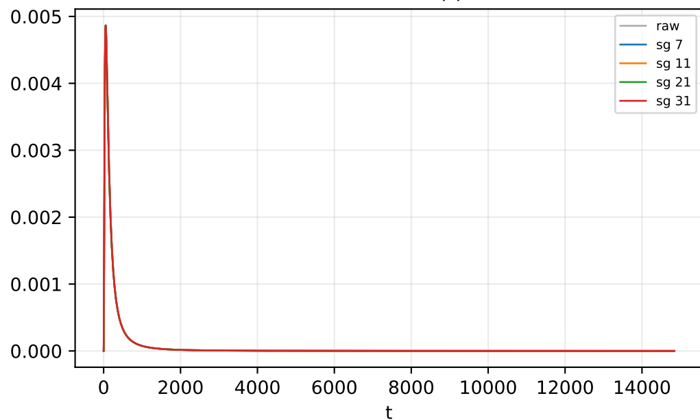
top f_k(t)
