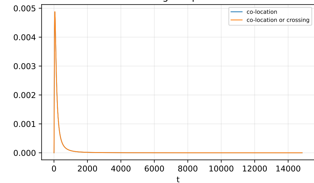
crossing comparison
