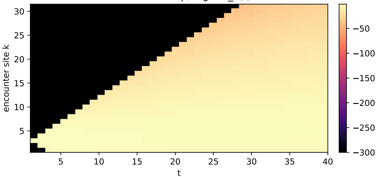
k-time heatmap, \log_{10} f_k(t)
