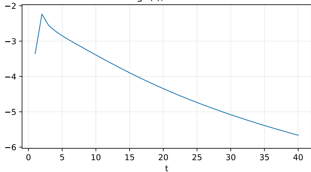
log-derivative of F2
