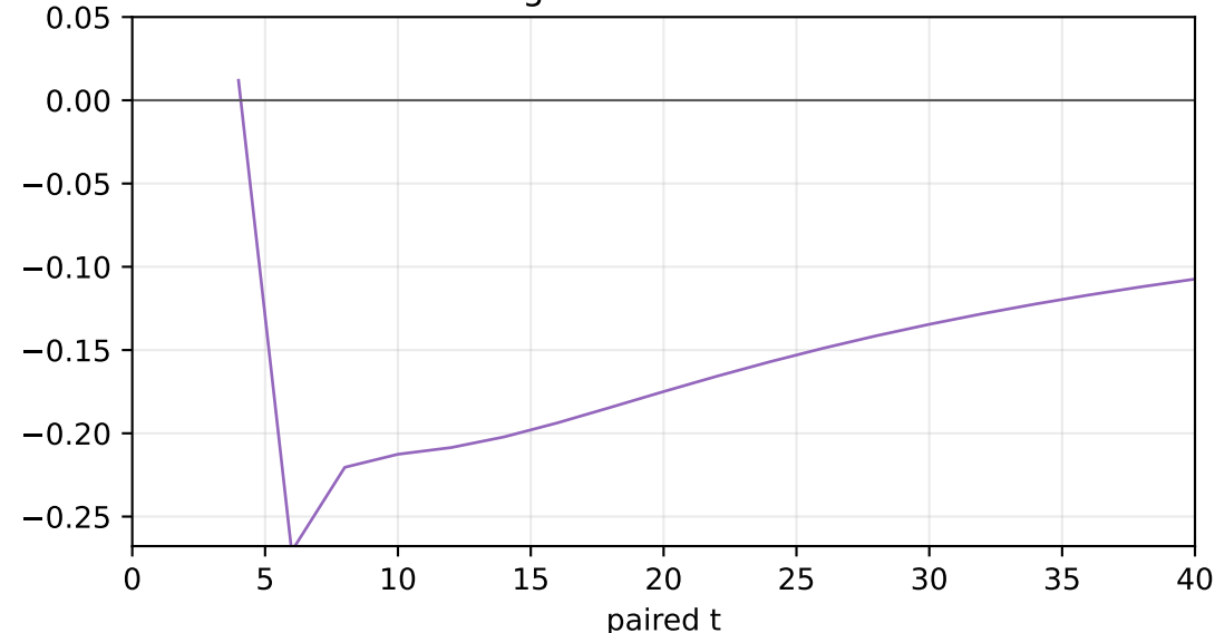
early/late encounter-site C_k
