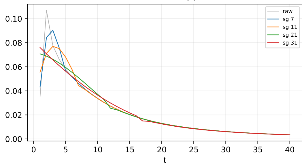
log f(t) , zoomed
