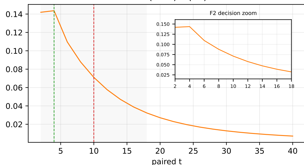
hazard h(t)=f(t)/S(t-1)
