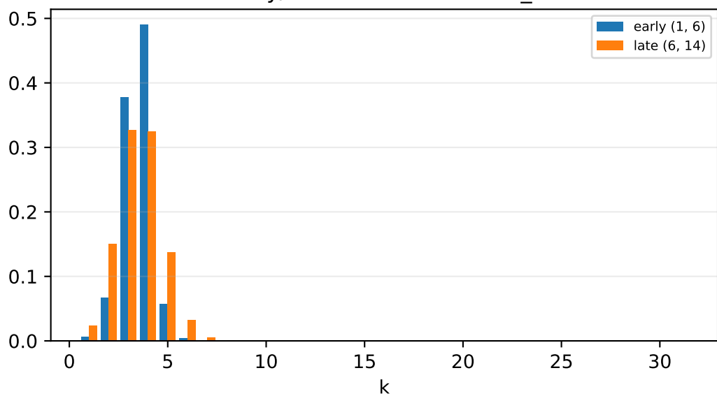
early/late encounter-site C_k
