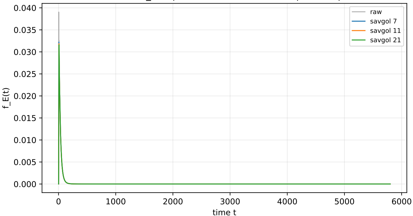
smoothed local_bump: N=21, start=(20, 16), q1=0.9, q2=0.02
