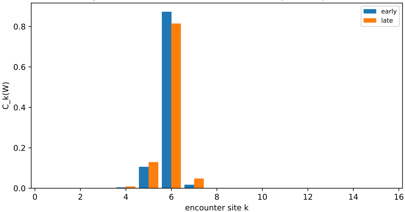
early vs late channels: N=15, start=(2, 6), q1=0.9, q2=0.02
