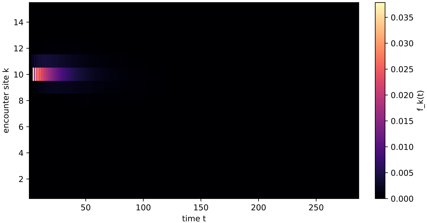
k-time heatmap: N=15 , start=(14, 10), q_1=0.9 , q_2=0.02
