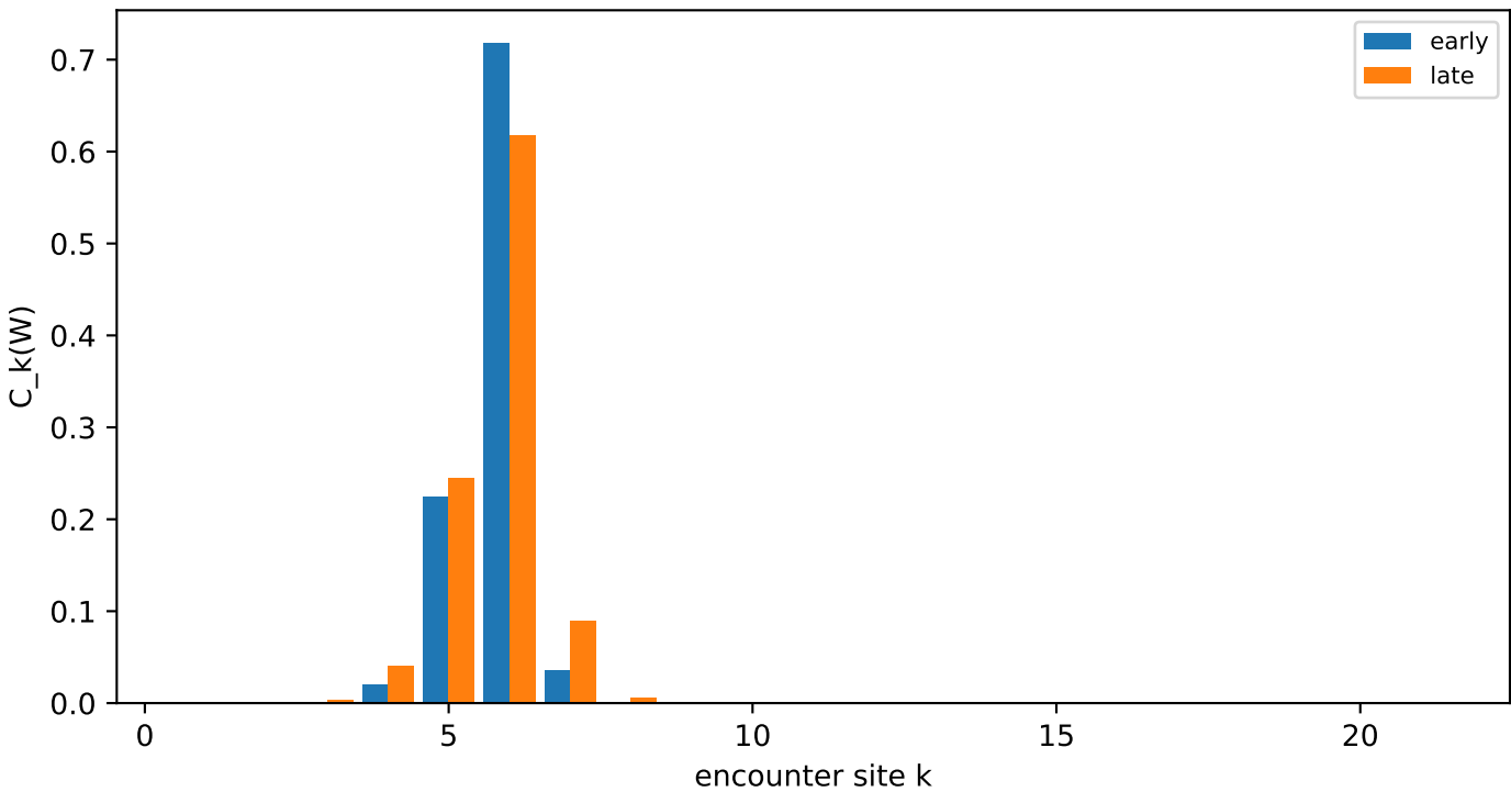
early vs late channels: N=21 , \text{start}=(2, 6) , q_1=0.9 , q_2=0.05
