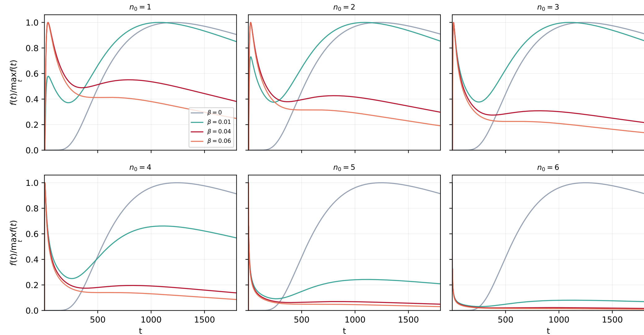
Shape comparison of representative first-passage curves
