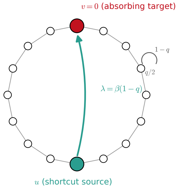
(a) lazy ring, N sites, directed shortcut
