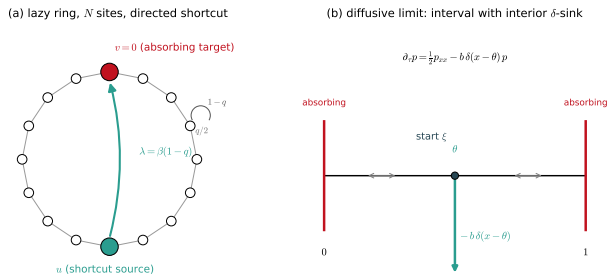
FIG. 1. Model. (a) Lazy random walk on a ring of N sites (stay 1-q , hop q/2 ) with an absorbing target v=0 and a directed shortcut u \rightarrow v of rate \lambda = \beta(1-q) ; deleting v leaves a rank-one killing defect at u . (b) Diffusive limit: Brownian motion on [0, 1] with absorbing ends and an interior \delta -sink of strength b at \theta , started at \xi .
