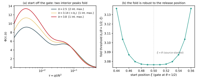
FIG. 5. Start dependence (Sec. IV E). (a) Continuum FPT density \Phi(\tau; b) for a walker released off the gate ( \xi = 0.44 , \theta = \frac{1}{2} ): both the capture and the diffusive-return features are genuine interior peaks, which annihilate through the fold as b crosses b_c \simeq 3.14 (two interior maxima \rightarrow one). (b) The fold threshold b_c(\theta = \frac{1}{2}; \xi) varies smoothly and symmetrically about the source-started point \xi = \theta , so the saddle-node is robust to the release position.
