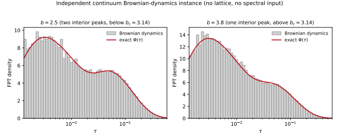
FIG. 4. Independent instance. A continuum Brownian-dynamics simulation of the delivery-gate protocol ( 6 \times 10^4 walkers, Euler-Maruyama, gate width \ell = 0.02 , \theta = \frac{1}{2} , start \xi = 0.44 ; no lattice, no spectral input) reproduces the exact \delta -sink density \Phi(\tau) (red) and the fold: two interior peaks below b_c \simeq 3.14 (left) and one above (right).
