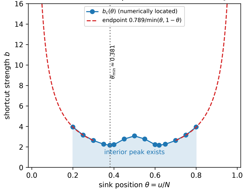
(a) saddle-node phase boundary b_c(\theta) (finite-time interior peak exists for 0 < b < b_c )
