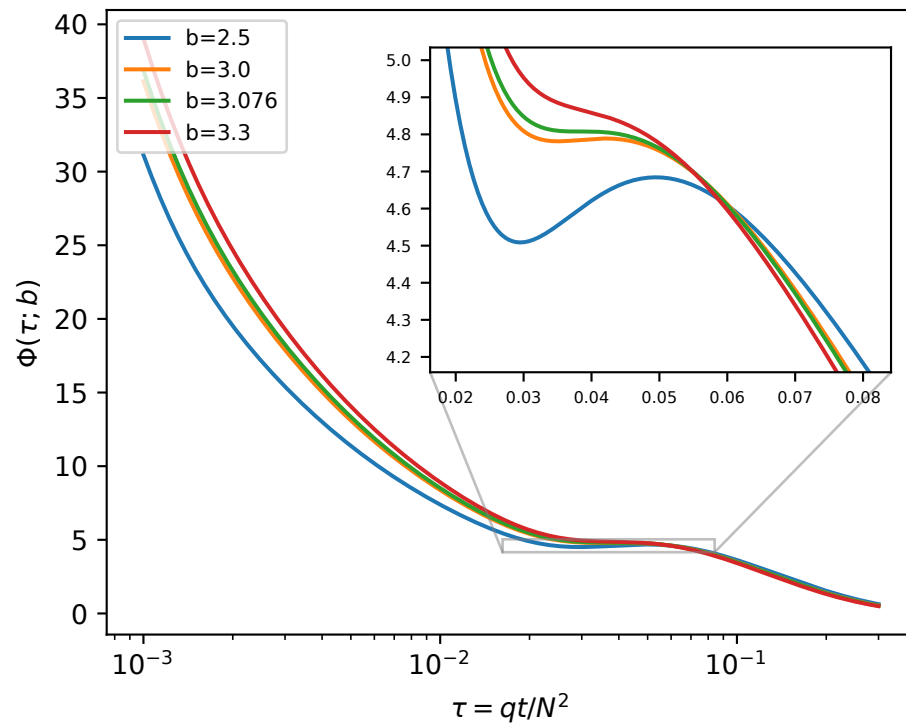
(b) master curve \theta = \xi = 1/2 : finite-time peak annihilates at b_c = 3.0764
