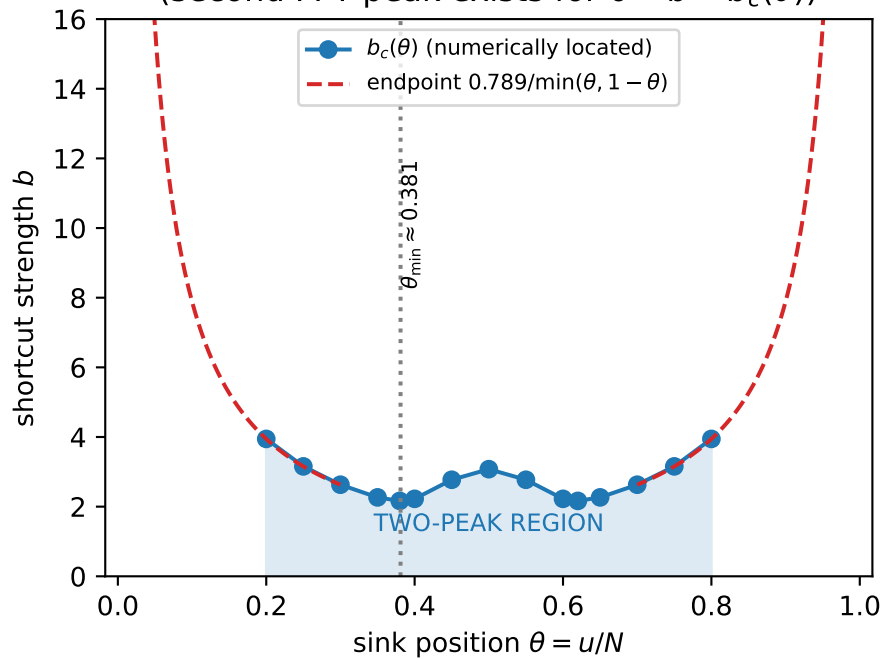
A. Saddle-node phase boundary (second FPT peak exists for 0 < b < b_c(\theta) )
