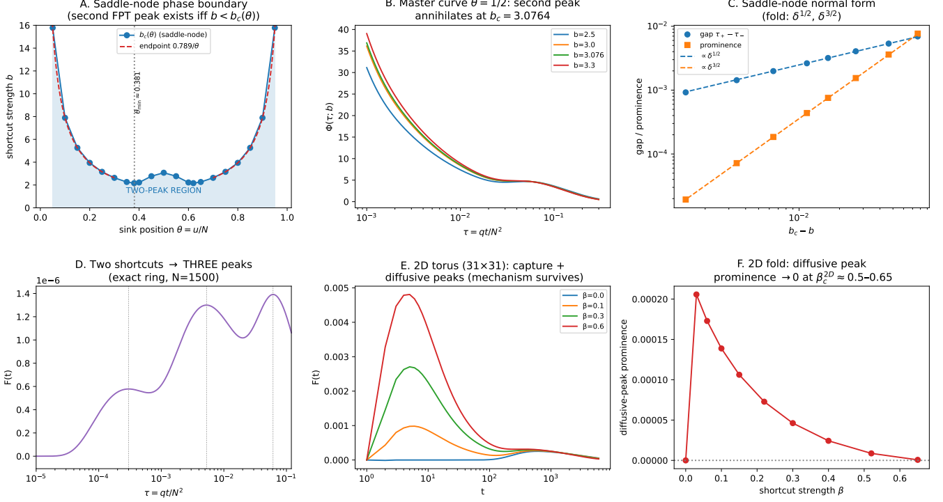
FIG. 2. Results. (a) Saddle-node phase boundary b_c(\theta) : the second FPT peak exists for 0 < b < b_c(\theta) ; symmetric, minimum at \theta \simeq 0.381 , with the endpoint law 0.789/\theta (dashed). (b) Master curve \Phi(\tau; b) at \theta = \frac{1}{2} as b crosses b_c = 3.0764 . (c) Normal-form scaling: gap \propto (b_c - b)^{1/2} and prominence \propto (b_c - b)^{3/2} . (d) Two shortcuts produce a third peak (exact ring, N = 1500 ). (e) 2D torus ( 31 \times 31 ): capture and diffusive peaks. (f) 2D fold: the diffusive-peak prominence vanishes at \beta_c^{2D} \simeq 0.55\text{--}0.65 .
