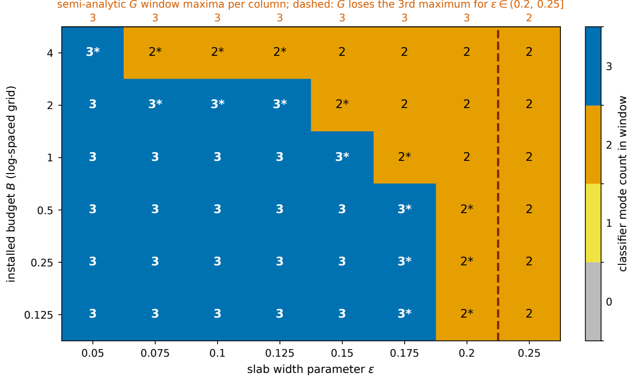
FIG. 2. Operational modality phase diagram for the m = 3 design at equal slab weights: colour and printed number give the classifier mode count in each (\varepsilon, B) cell ( 10^6 walkers; * = verdict-boundary-adjacent cells re-run at 3 \times 10^6 walkers, none of the sixteen changing verdict); blue marks cells retaining all three modes, orange cells that lost one. The retained-mode boundary is a monotone staircase in (\varepsilon, B) ; the dashed line marks the B -independent semi-analytic boundary \varepsilon \in (0.2, 0.25] beyond which the free exposure clock G itself loses its third window maximum. The \varepsilon = 0.2 column sits at the classifier floor (Sec. IVD). (Plotting code revised with Codex assistance; numerical content author-verified.)
