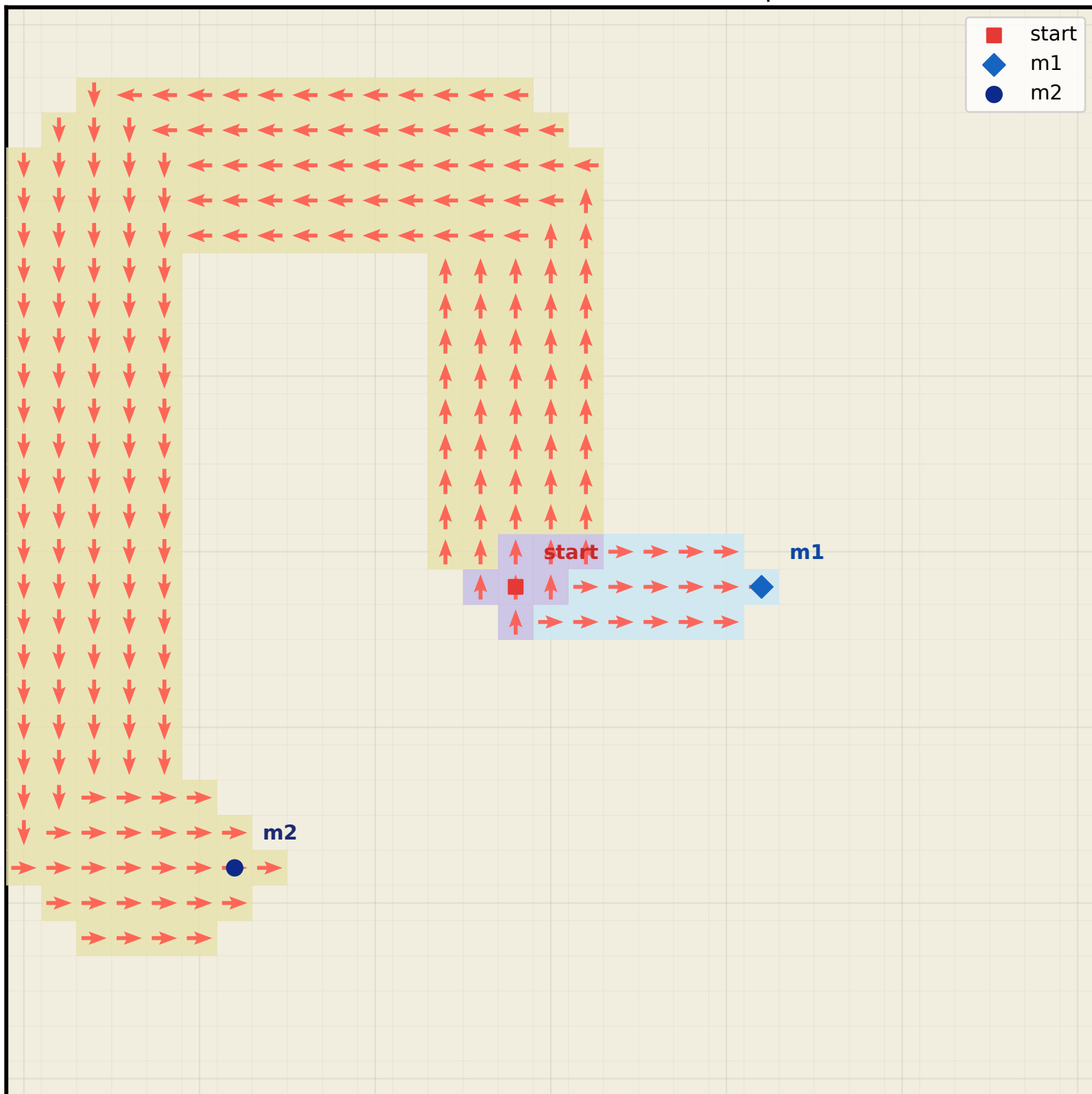
C2: full local-bias arrow field (w2=2, skip2=1)
