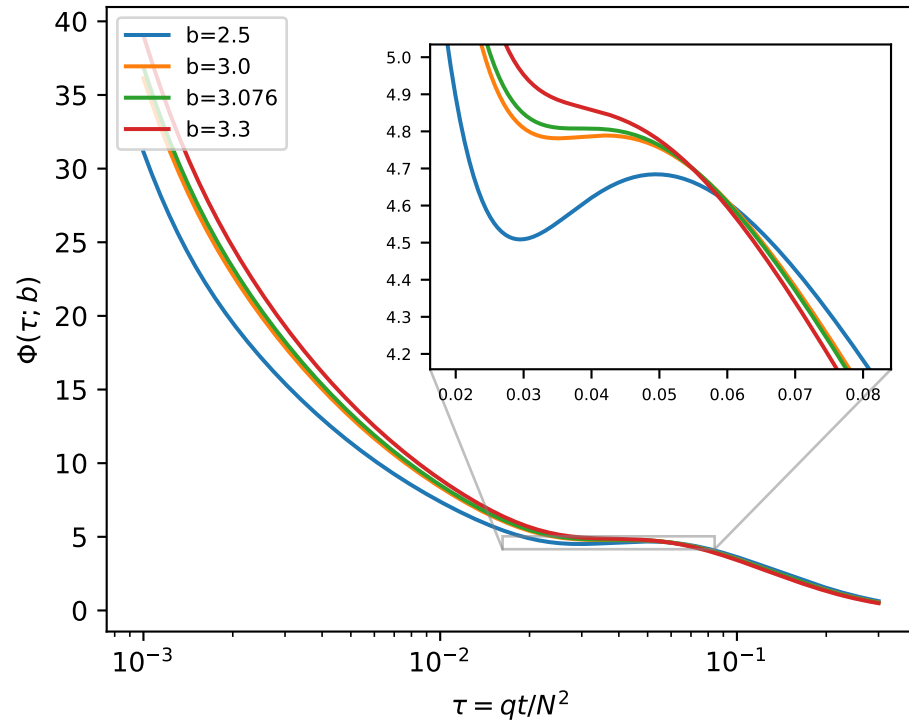
(b) master curve \theta = \xi = 1/2 : second peak annihilates at b_c = 3.0764
