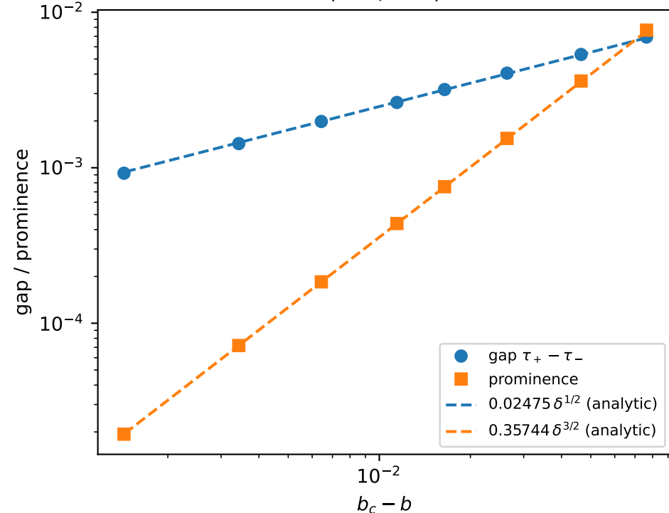
(c) normal-form fold scaling ( \delta^{1/2} , \delta^{3/2} )
