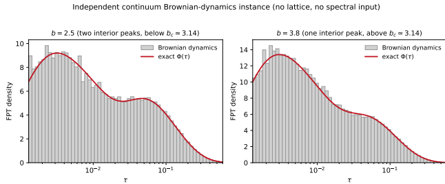
FIG. 5. Direct stochastic realization. A continuum Brownian-dynamics simulation of the delivery-gate protocol ( 6 \times 10^4 walkers, Euler-Maruyama, gate width \ell = 0.02 , \theta = \frac{1}{2} , start \xi = 0.44 ; no lattice, no spectral input) reproduces the exact \delta -sink density \Phi(\tau) (red) and the fold: two interior peaks below b_c \simeq 3.14 (left) and one above (right).
