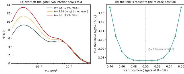
FIG. 4. Start dependence (Sec. IV A). (a) Continuum FPT density \Phi(\tau; b) for a walker released off the gate ( \xi = 0.44 , \theta = \frac{1}{2} ): both the capture and the late (indirect) features are genuine interior peaks; the late peak and its valley annihilate through the fold as b crosses b_c \simeq 3.14 (two interior maxima \rightarrow one). (b) The fold threshold b_c(\theta = \frac{1}{2}; \xi) varies smoothly and symmetrically about the source-started point \xi = \theta , so the saddle-node is robust to the release position in a neighborhood of the gate.
