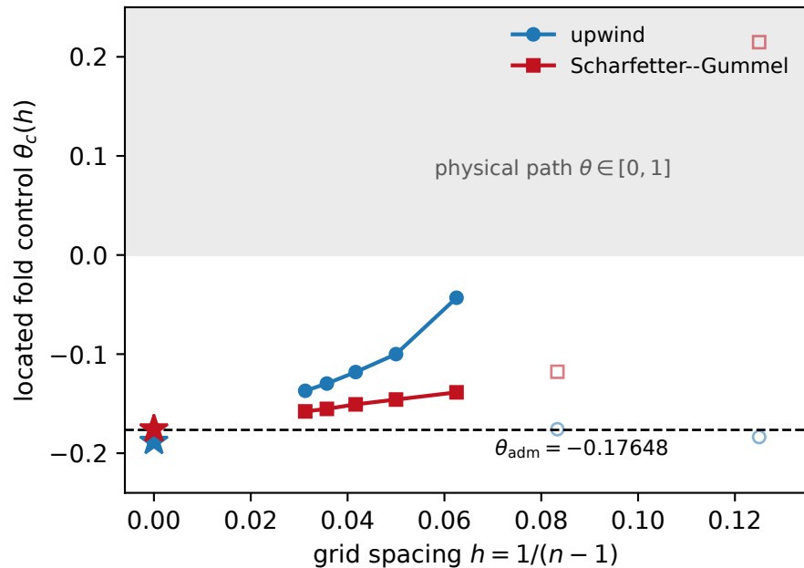
(a) refinement ladder: fold outside the physical path
