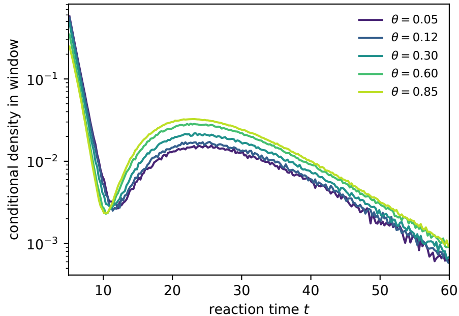
(b) off-lattice realization: late maximum on the path
