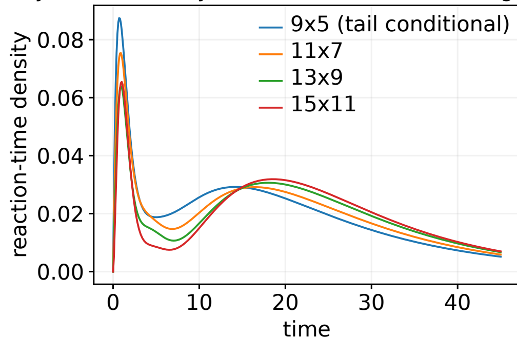
(b) bimodality across four declared finite grids
