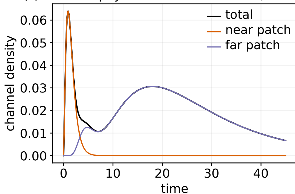
(c) resolved physical reaction channels, 13x9 grid
