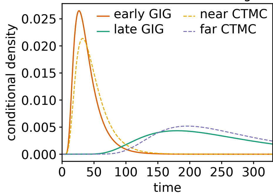
C Physical CTMC fold
