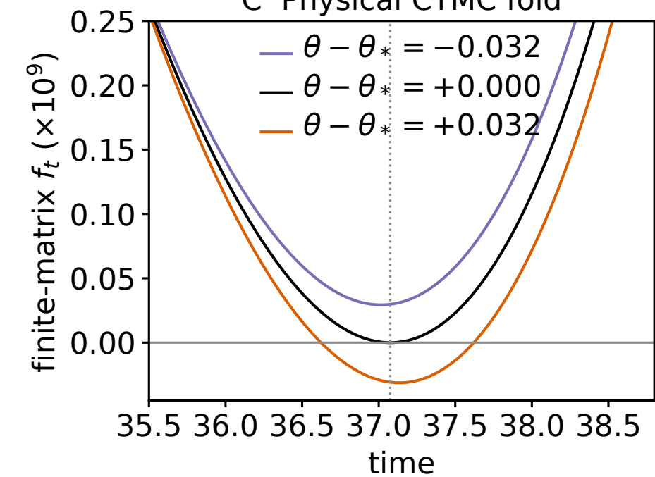
C Physical CTMC fold
