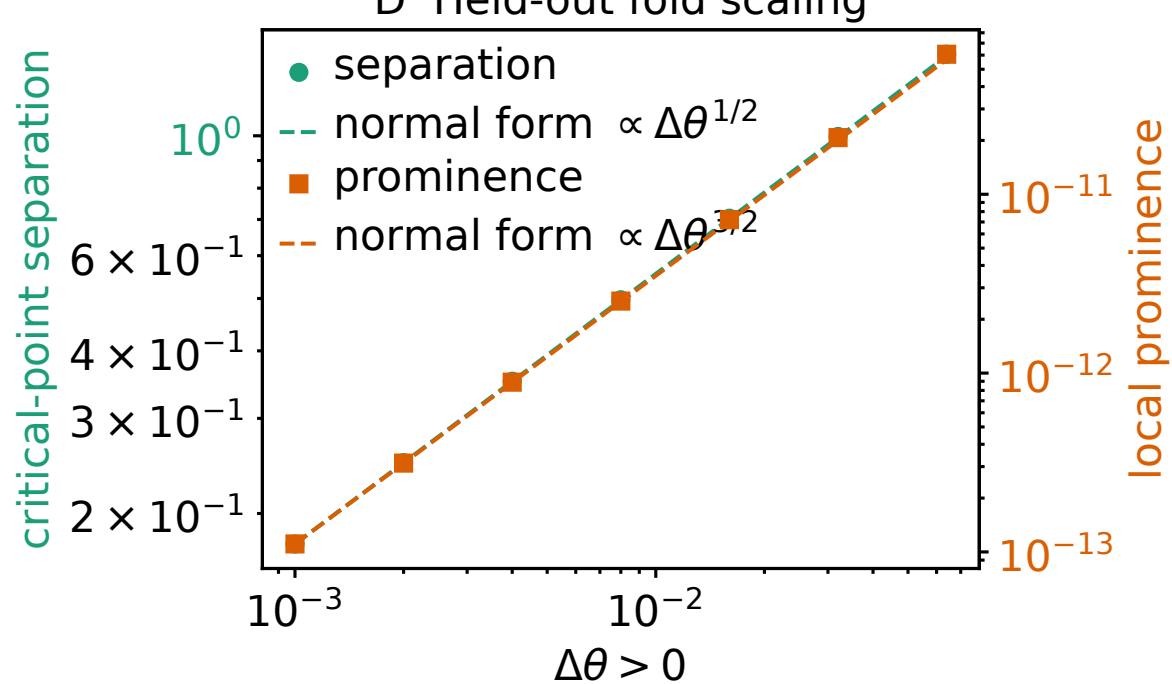
D Held-out fold scaling
