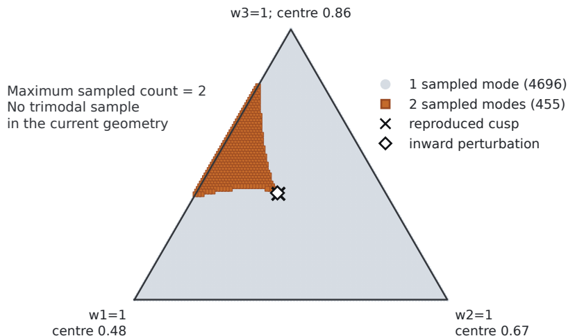
(c) Sampled catalyst-weight simplex 5151 controls; weight and time spacing 0.01
