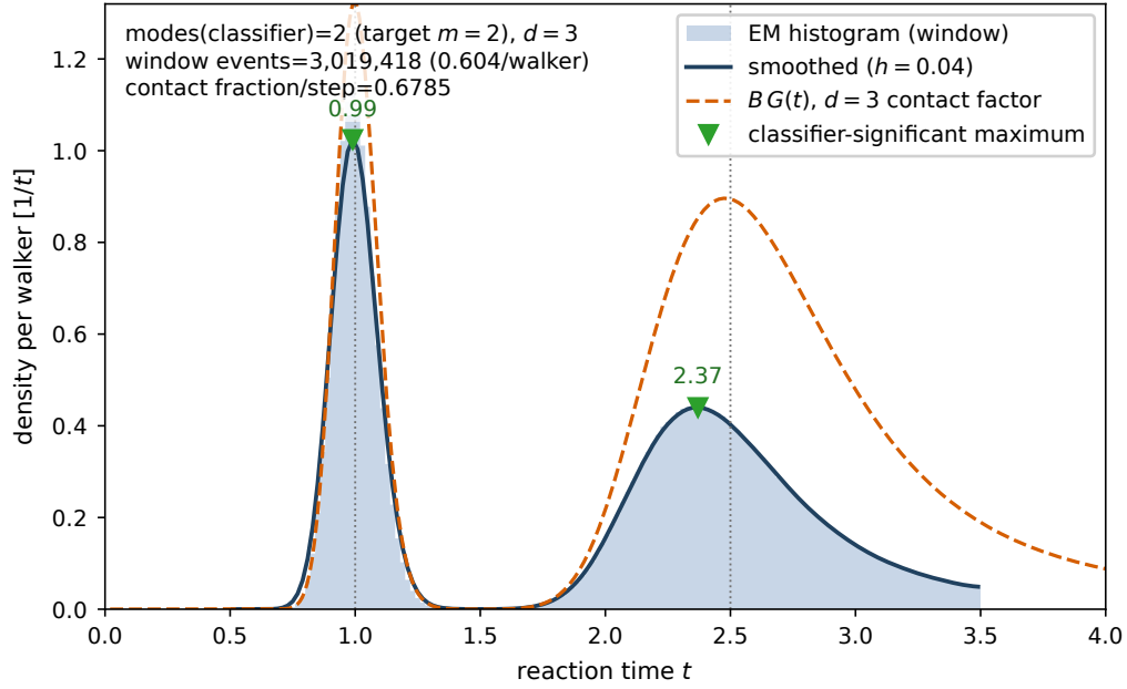
FIG. S3. d = 3 spot check: two transverse torus directions, killing prefactor B/W^2 , all remaining parameters unchanged from the (m, \varepsilon, B) = (2, 0.1, 1) anchor. The fixed classifier identifies two significant modes at t = 0.99 and 2.37 , with 0.60 reaction events per walker inside the window and \Delta t -halving maximum |z| = 1.67 . (Plotting code revised with Codex assistance; numerical content author-verified.)
