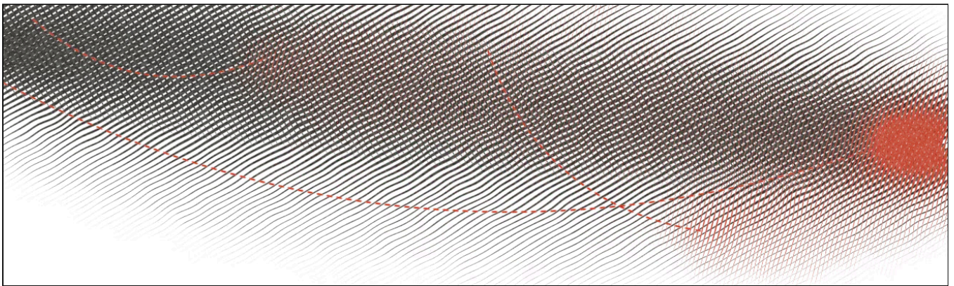
FIG. 0 The Plate – 2021 to now, as a long exposure. Toy model: walkers drift toward the event you choose; shortcuts jump. Red = took a shortcut (fast). Silver = the long way (slow). The paper’s exact ring model is in Chapter 01.
